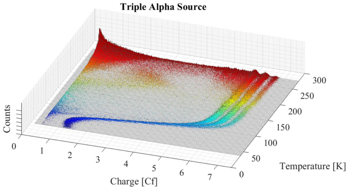
Figure 7.9 - Energy spectra collected from a triple alpha source from RT down to 46 K [95].
