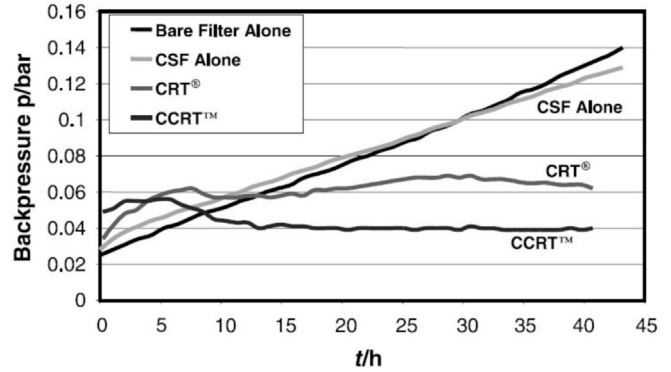
Fig. 31. Comparison of DPF filters (non-catalyzed DPF, CSF, CRT, and CCRT) and their back-pressure behaviors in low exhaust gas temperatures T < 270^\circ C , Gorsmann et al. (2005).
